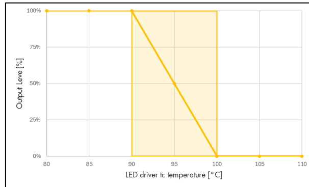
Image 35 – LED Driver OTP behavior
