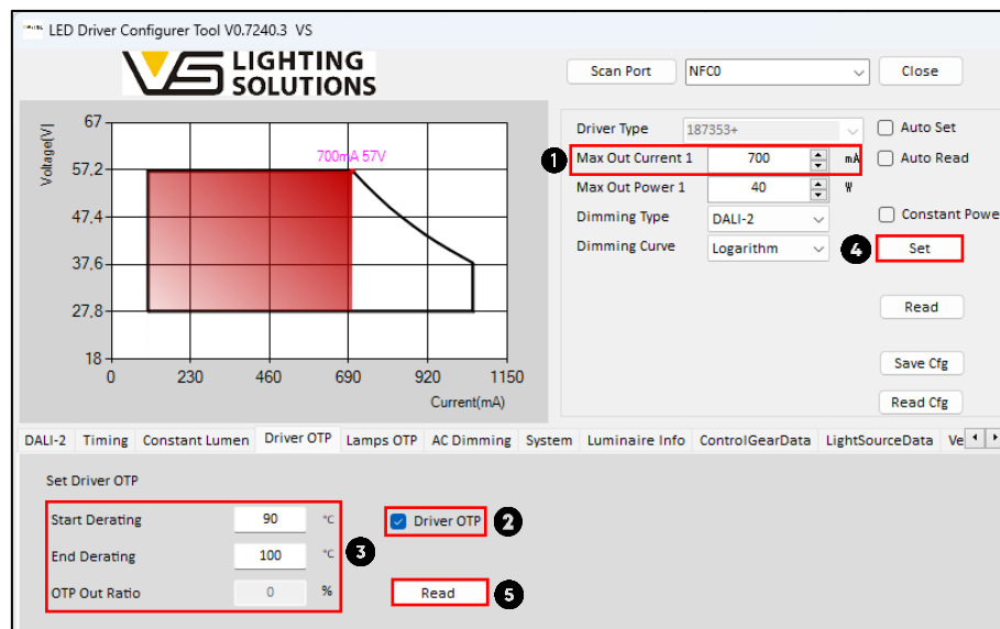
Image 34 – LED Driver OTP configuration
