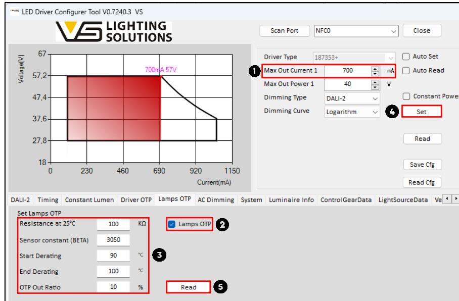
Image 36 – Luminaire OTP configuration
