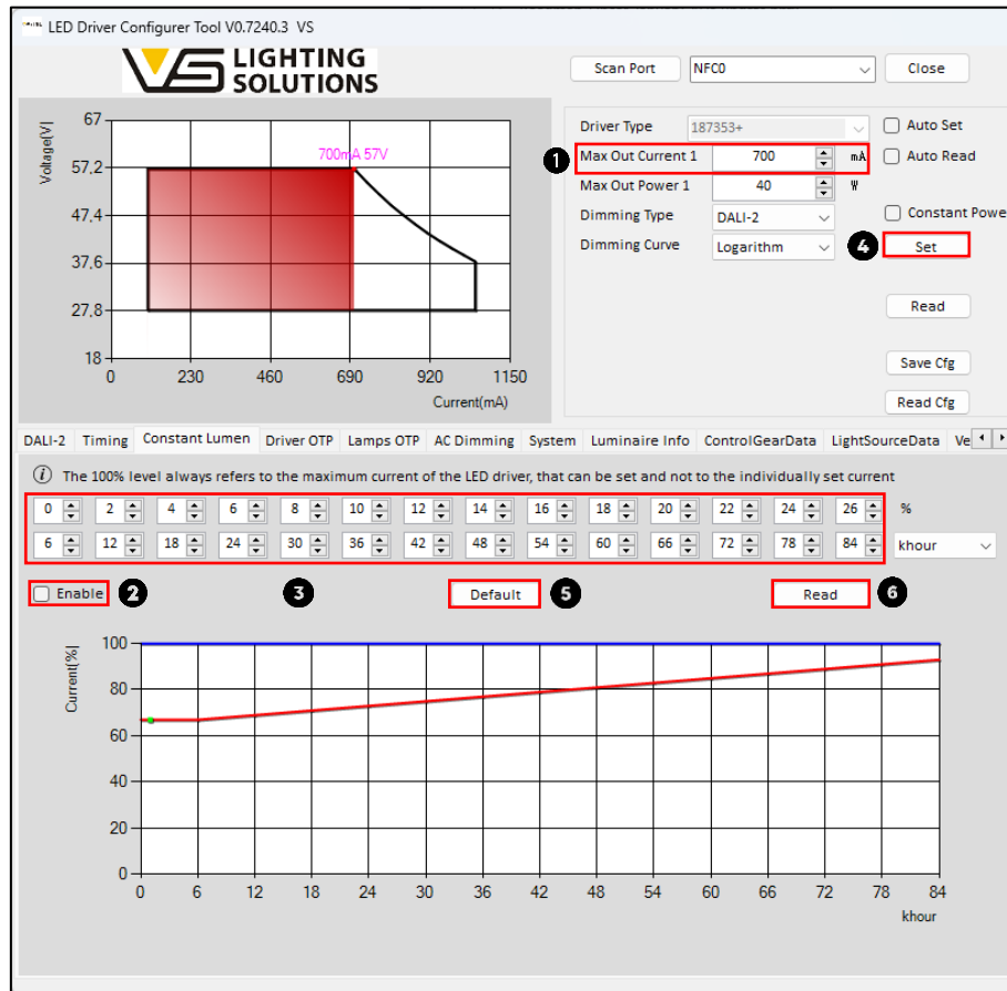
Image 33 – Constant lumen output configuration
